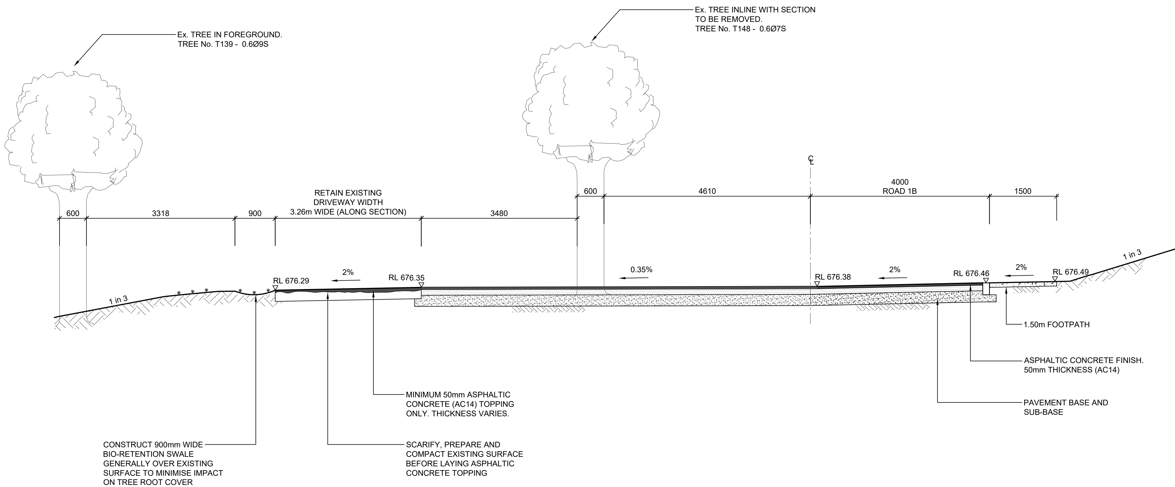
DETAILED SECTION AT CH 56.90 ROAD 1A & CH 40.0 ROAD 1B
